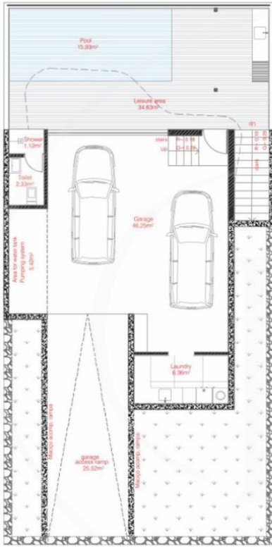
Basement esc: 1/100 VILLA DELTA
